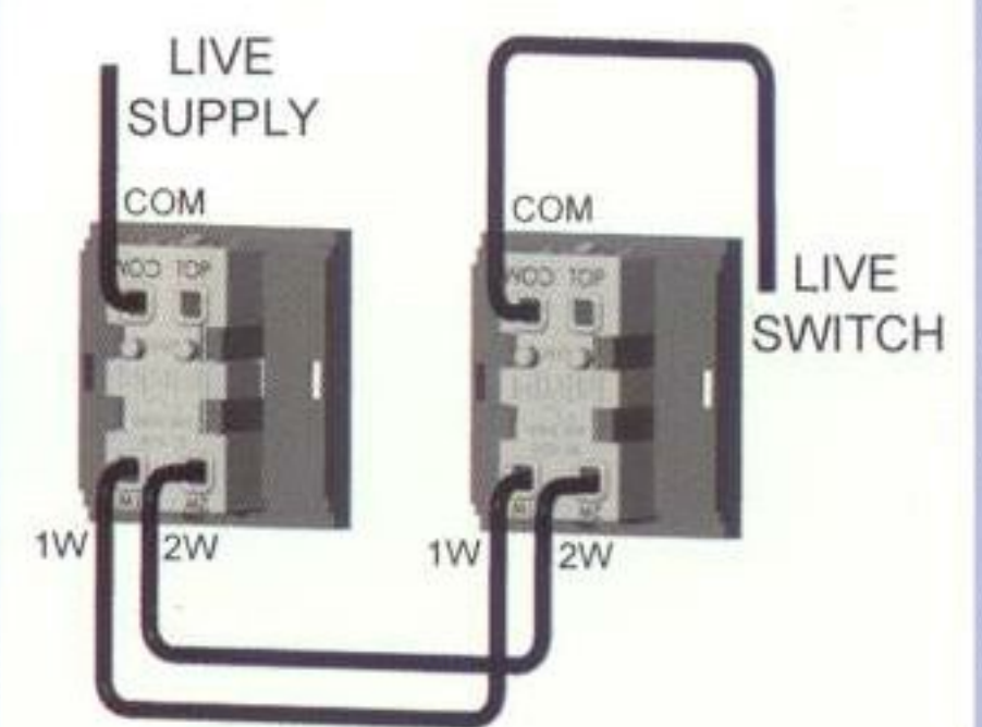
1 Gang 2 Way Loop In Loop Out
