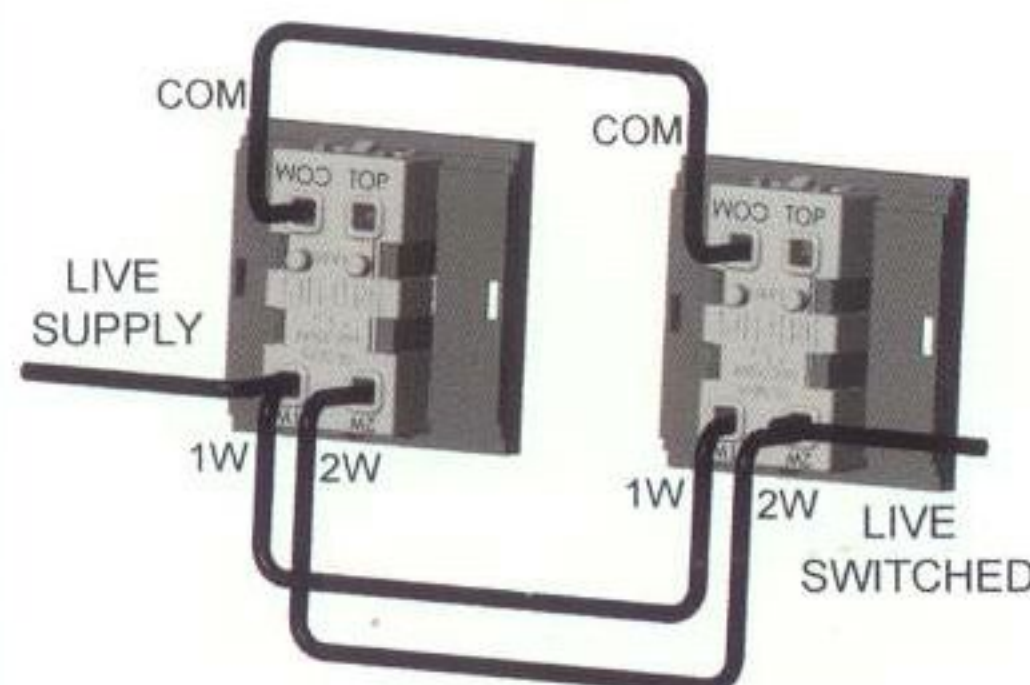
1 Gang 2 Way Alternative
