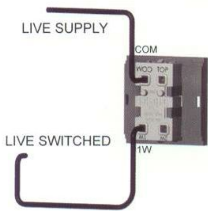
1 Gang 1 Way Switch
