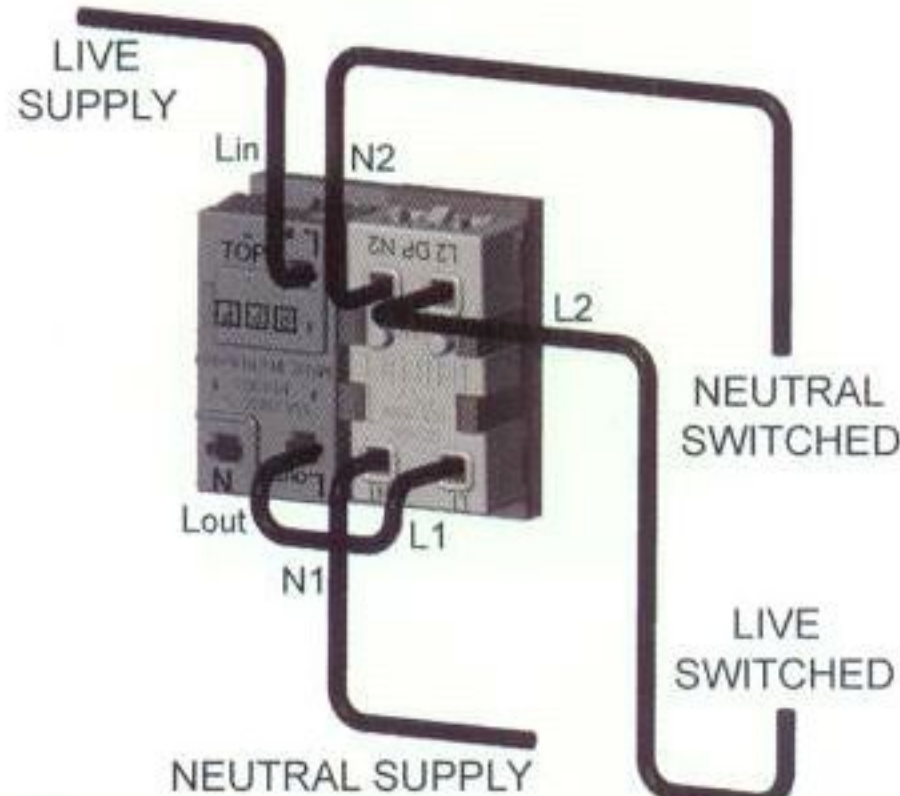
Switch Fuse Connection Unit
