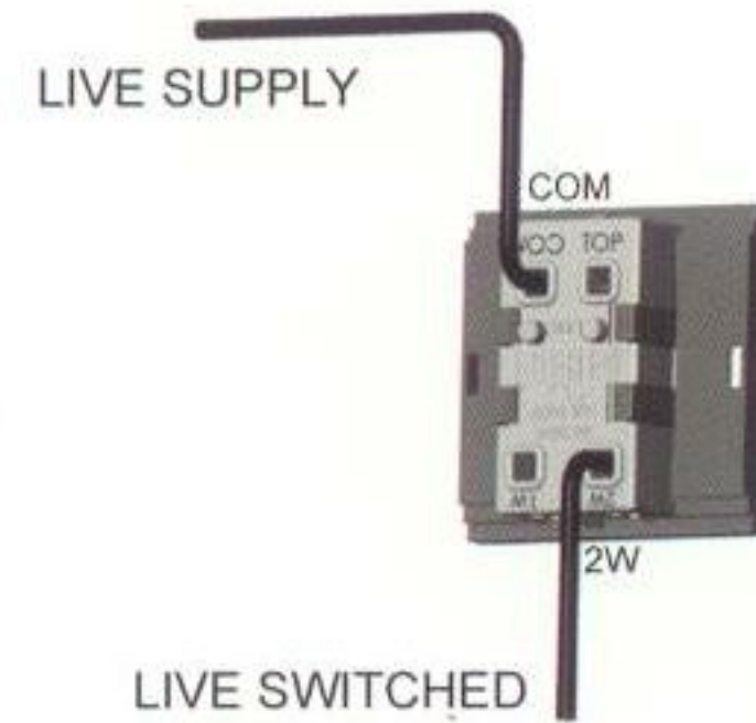
1 Gang Retractive (push to break)
