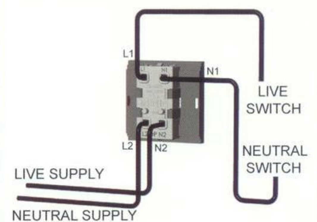
1 Gang Double Pole Switch
