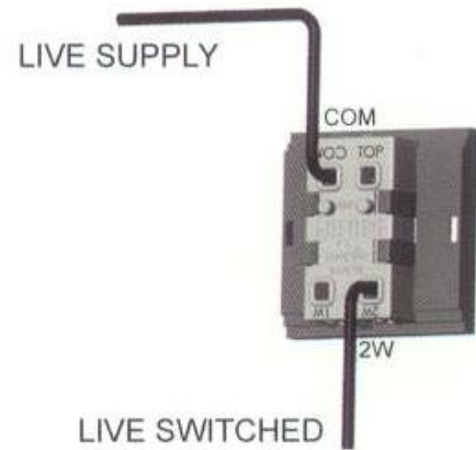
1 Gang Retractive (push to make)
